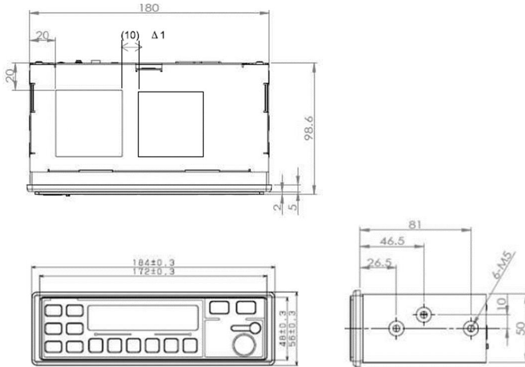
Figure 1 347-3110-000 Bluetooth radio Dimensions
