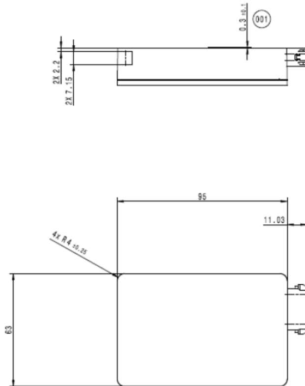
Figure.1 Dimensions
