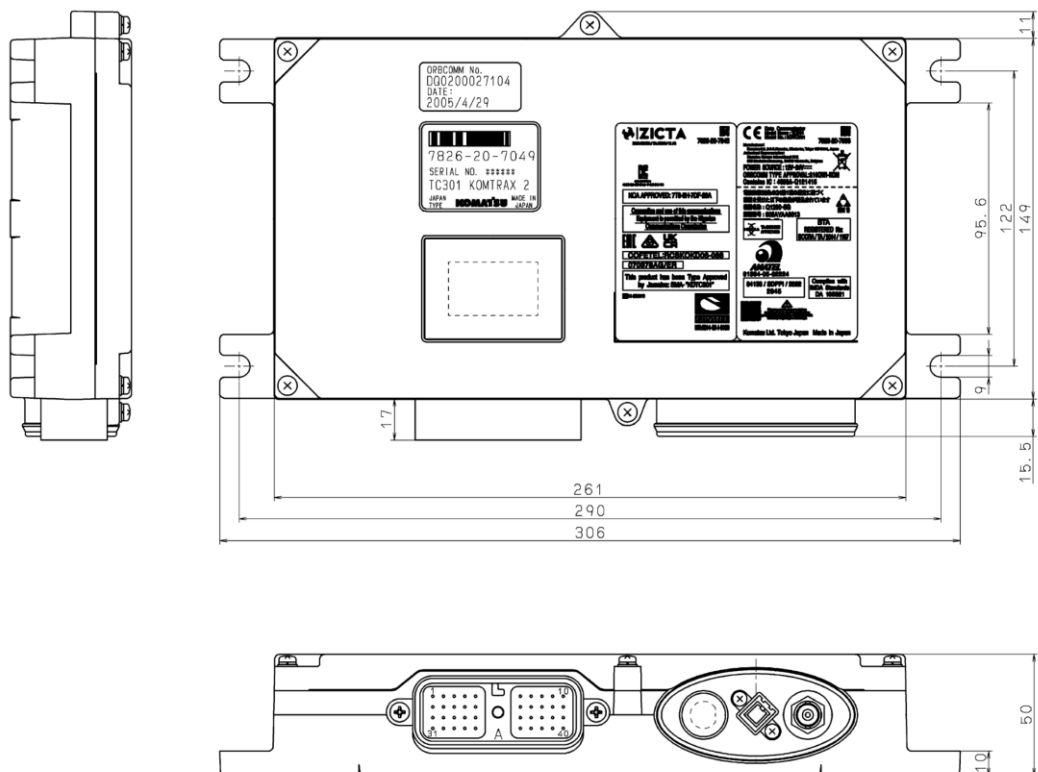
Figure 1 KDTC301 Dimensions
