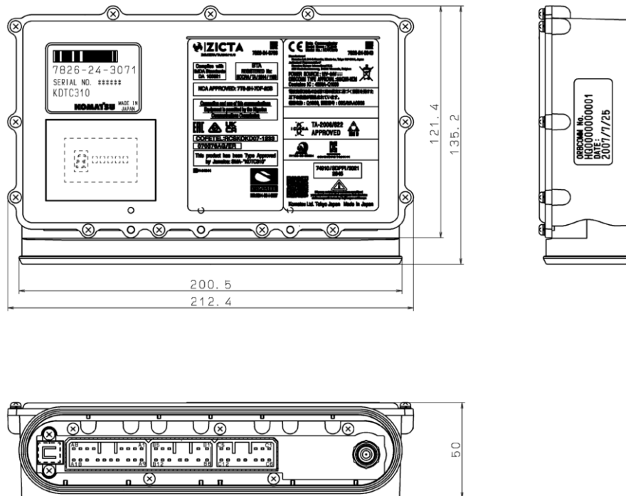
Figure 1 KDTC310 Dimensions
