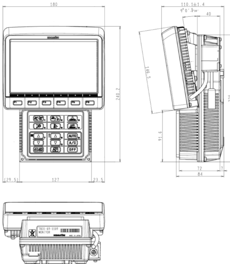
Figure 1 KDMH801 Dimensions
