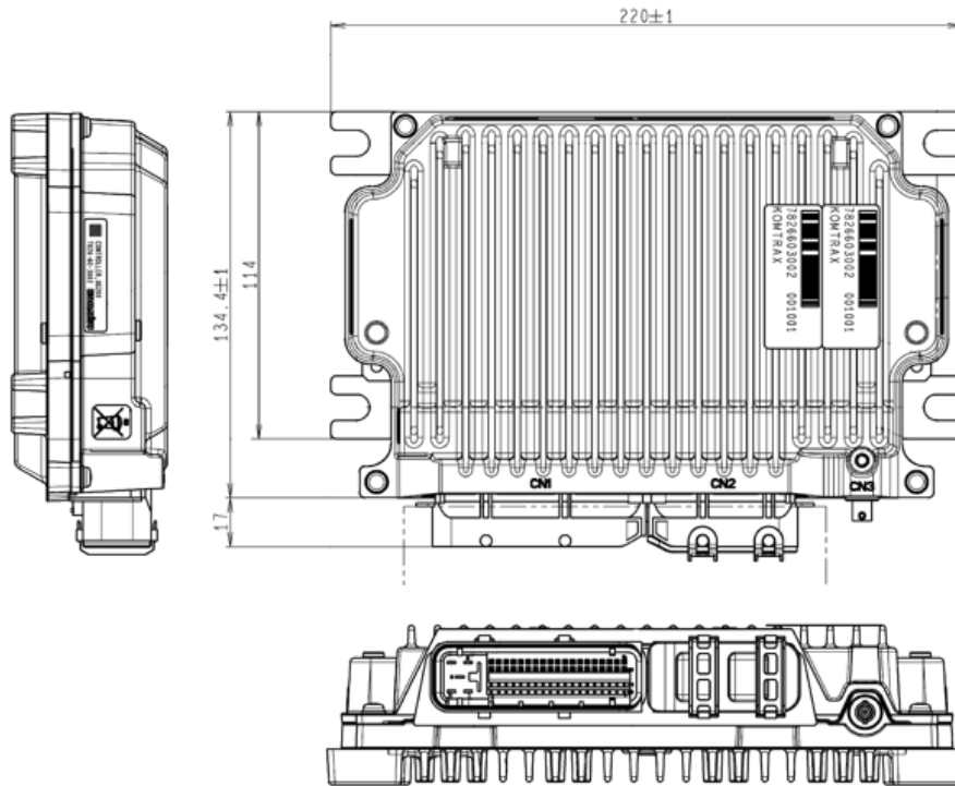
Figure 1 KDUG200 Dimensions
